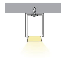
PROFILE ALUMINIUM FOR NEON 12×22mm RGBWW / 12×23mm RGB (14.5×19)
